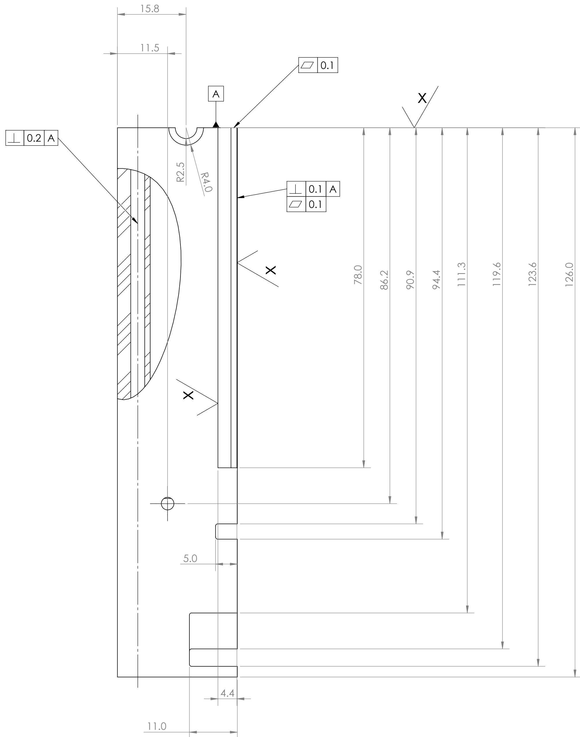
SECTION B-B
