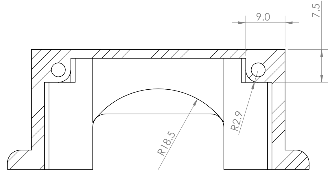
SECTION B-B
